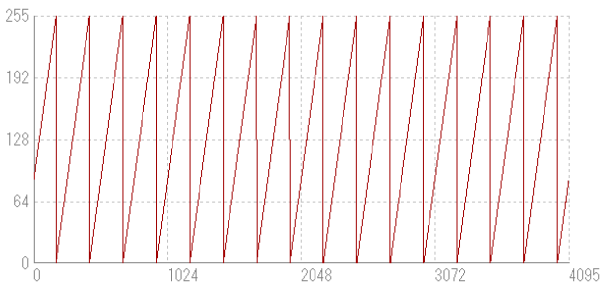
図 4-2-3-9(C) RCDL4K8GE NED_GreyDiagonalRamp
